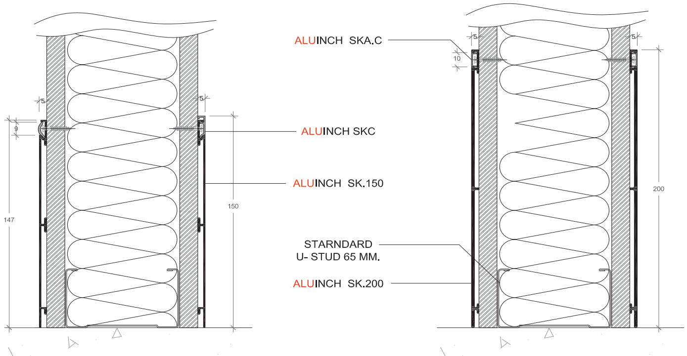
ALUINCH SK.150 150 MM. SCREW-ON SKIRTING
