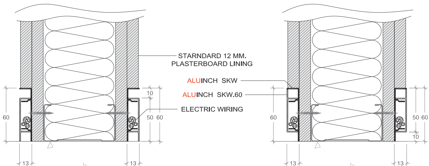
ALUINCH SKW OPTION 1 UPPER GROOVE
