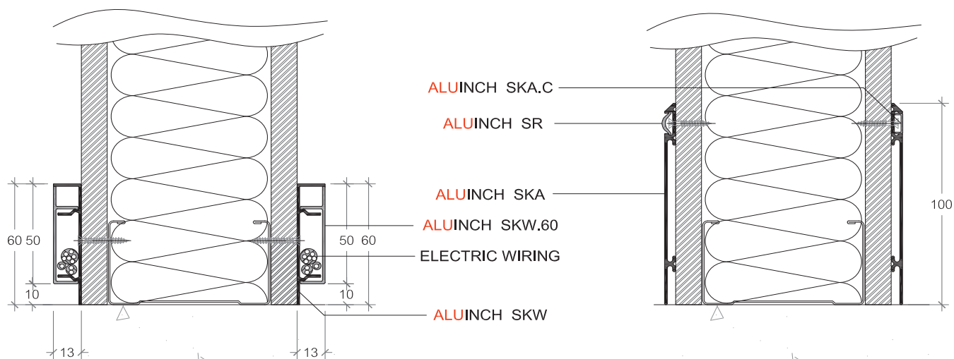
ALUINCH SKW OPTION 3 ON SURFACE
