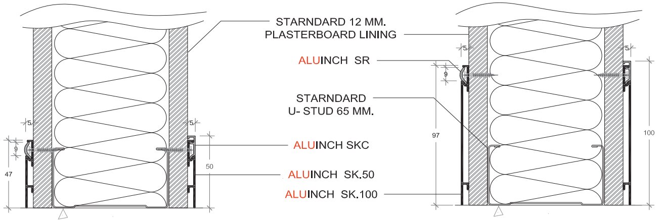
ALUINCH SK.100 100 MM. SCREW-ON SKIRTING
